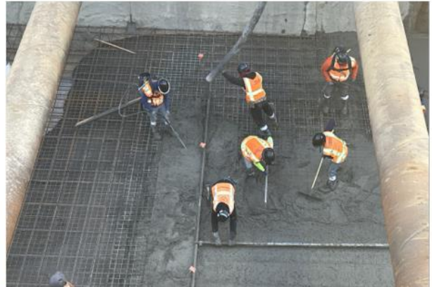
Concrete Placement of U-Wall Working Slab 3D
