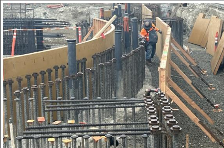
Formwork and Rebars for Cat Shaft Cap Beam Construction
