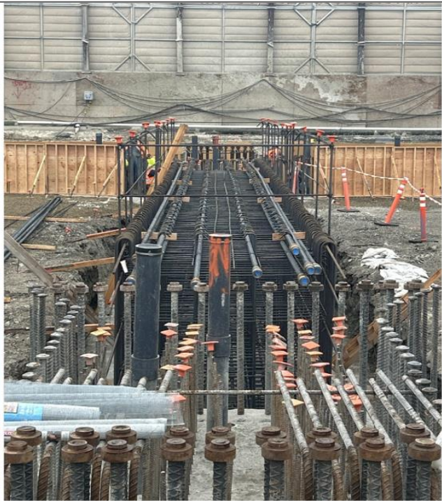
Rebars and Formwork for Construction of Cat Shaft Cap Beam and Top Strut
