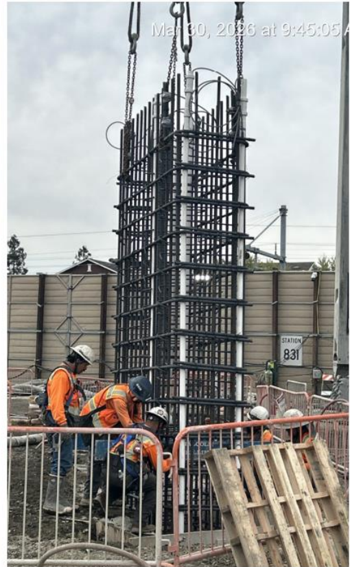
Cat Shaft Panel Rebar Cage Placement Operations
