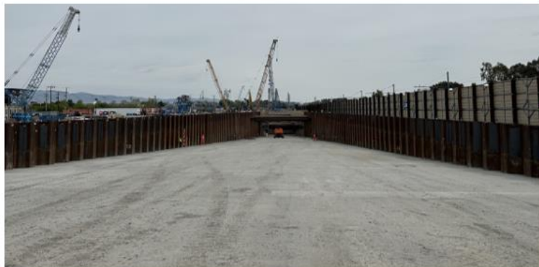
Bracing Elements Removed from Sheet Pile U-Wall
