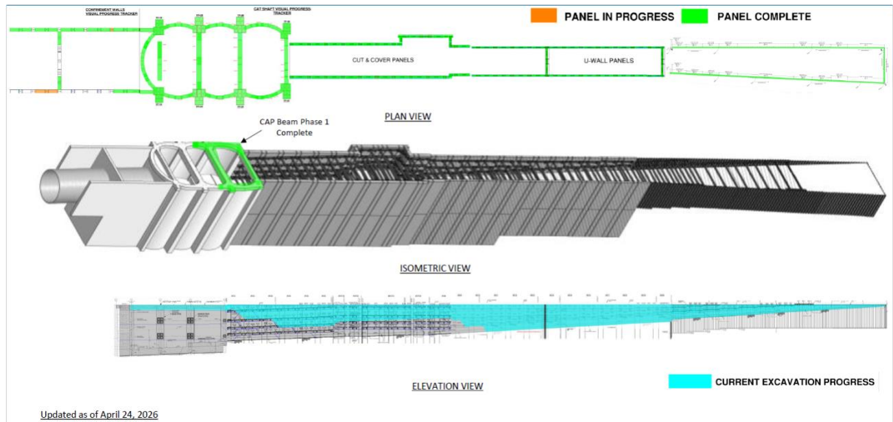
Figure 1 – Launch Structure Construction Progress tracker (as of April 24, 2026)
