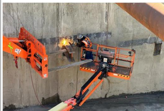
Removal of D-Wall Bracing Elements
