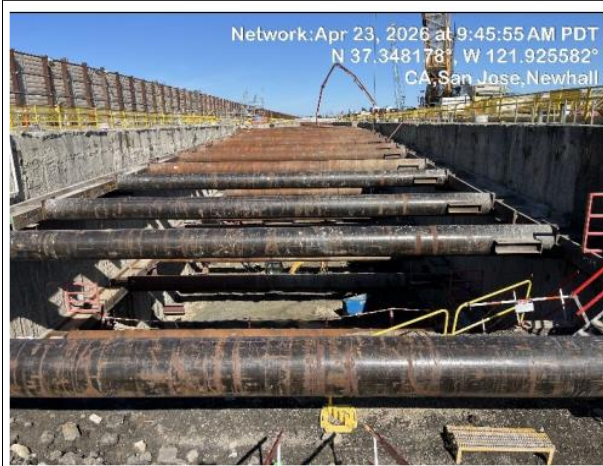
Overview of Level 1 Bracing of the SOE Structure
