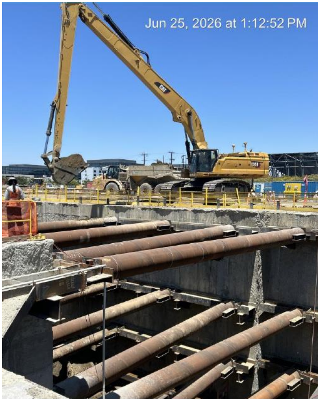
U-Wall – Subgrade Excavation
