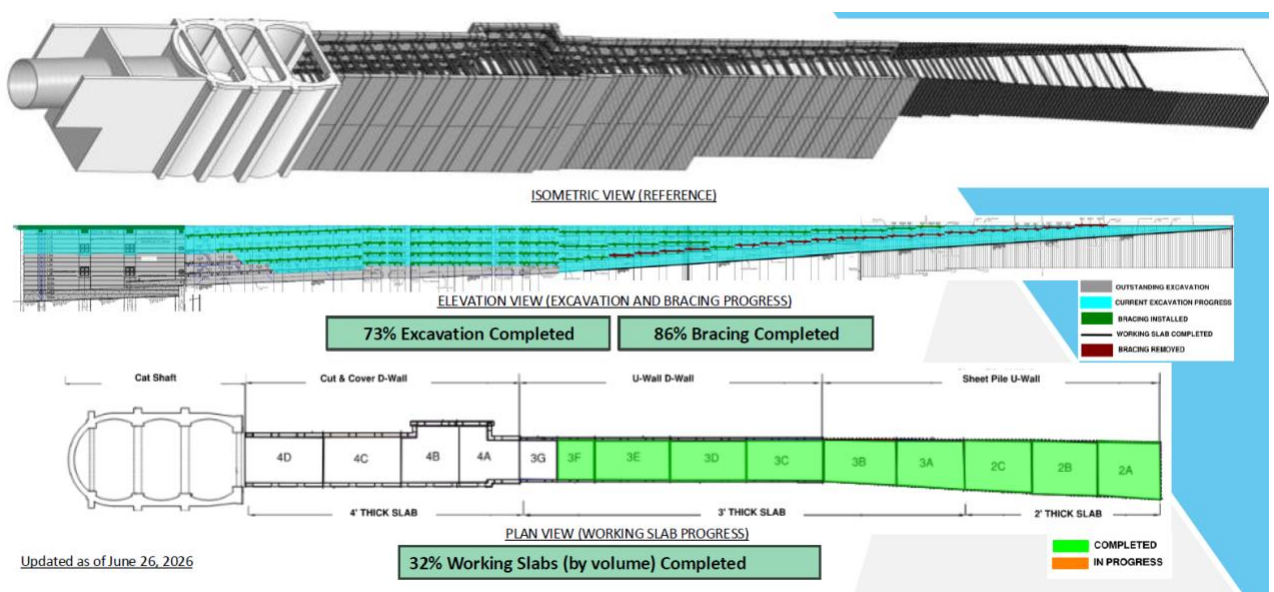
Figure 1 – Launch Structure Construction Progress tracker (as of June 26, 2026)
