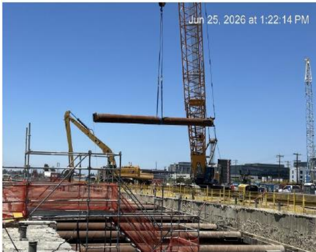
Cut & Cover – Level 4 Bracing Installation
