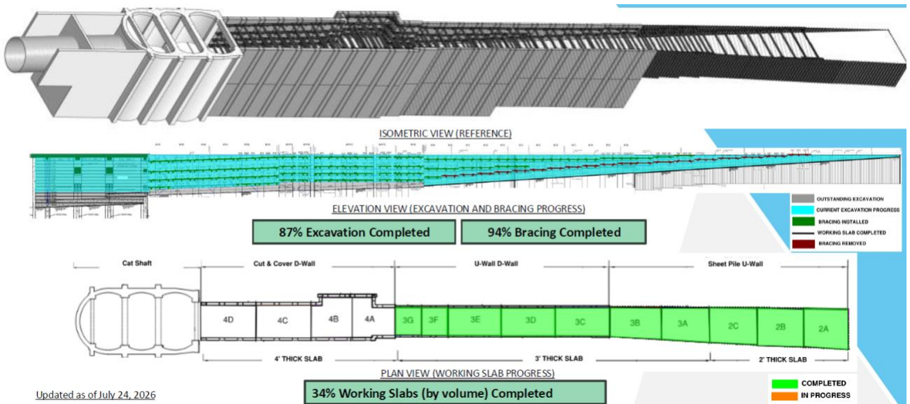
Figure 1 – Launch Structure Construction Progress tracker (as of July 24, 2026)
